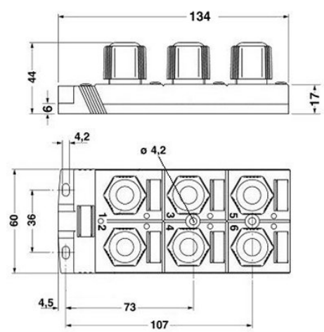
Dimensioned drawing
